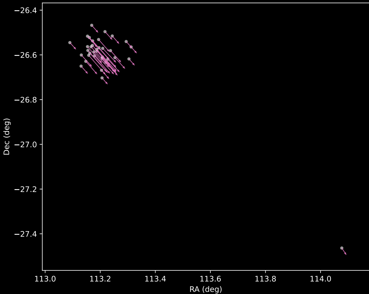
APOGEE DR17 Cluster 12 Proper Motion Vectors (n=35)
