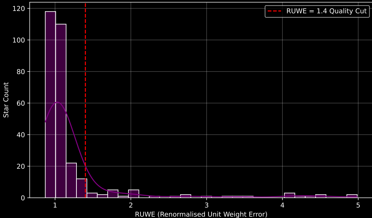
GAPOGEE DR17 Field [N288] RUWE Distribution (n= 295)
