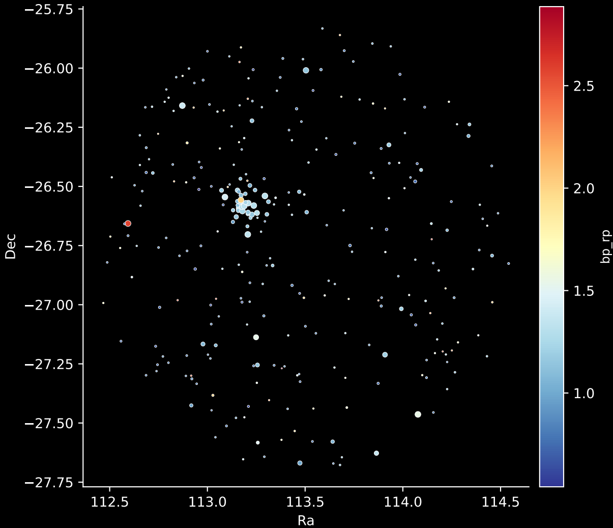
APOGEE DR17 Field: [N288] Stars: 306
