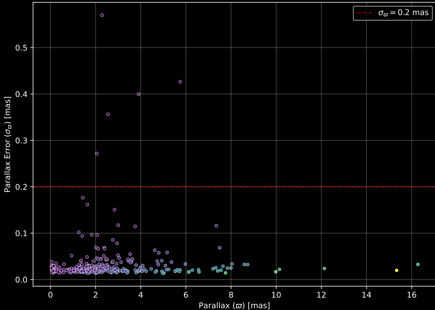
APOGEE DR17 Field: [N288] Parallax Quality (n= 306)
