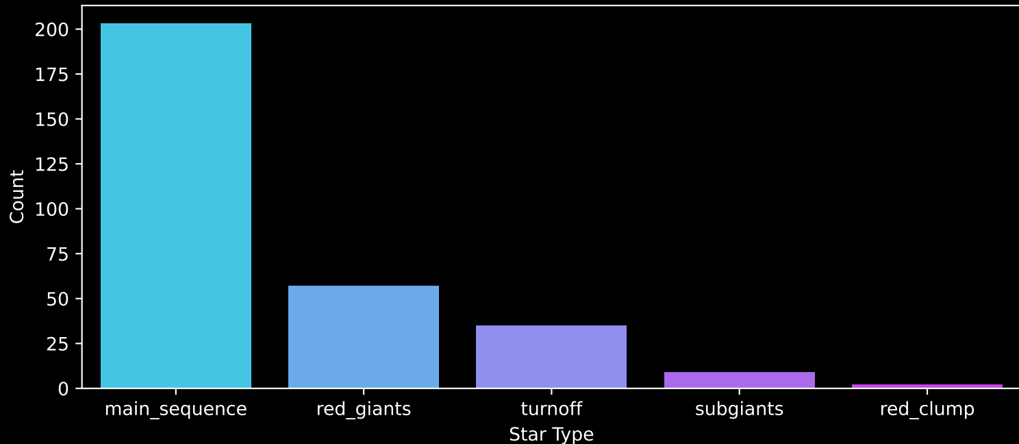
APOGEE DR17 Field: [N288] Count plot of Star Type
