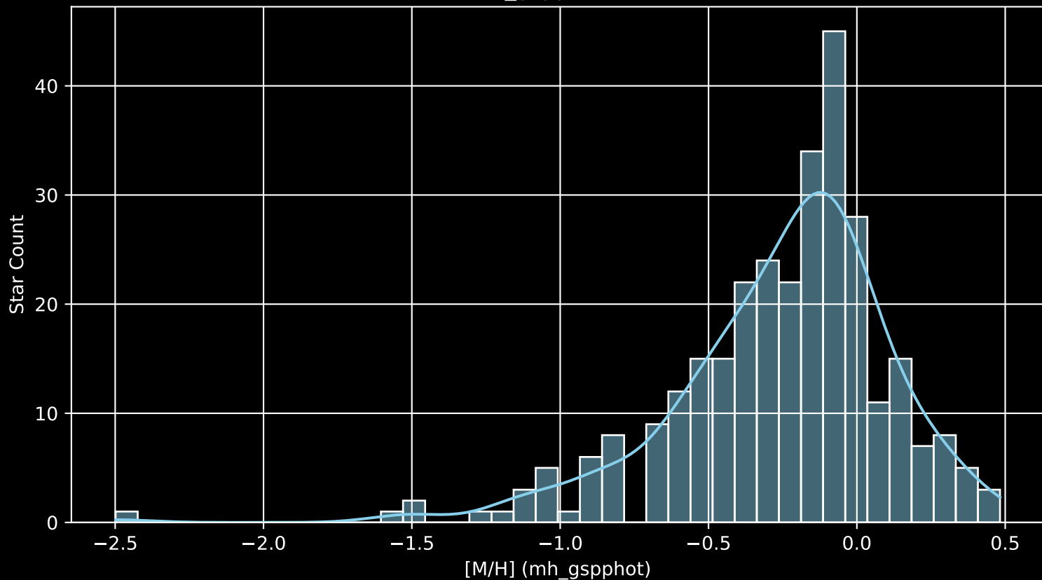
APOGEE DR17 Field: [N288 [M/H] (mh_gspphot) (n= 304)
