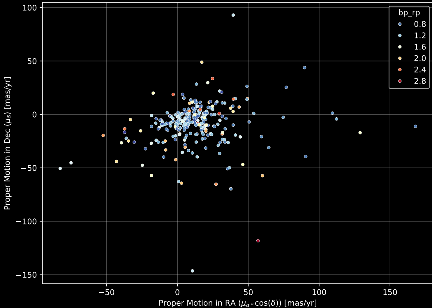
APOGEE DR17 Field: [N288] Proper Motion Diagram (n= 306)
